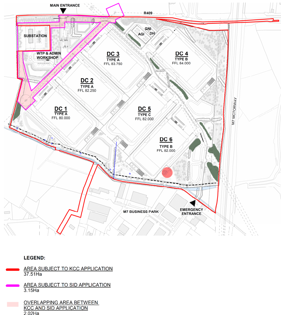
Figure 3-2. Proposed Concept Masterplan Source: RKD Architecture
